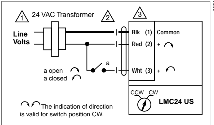
On-off control
