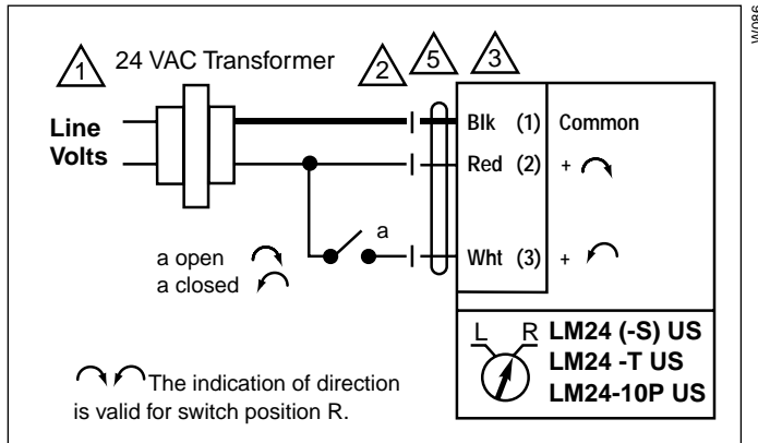
On-off control
